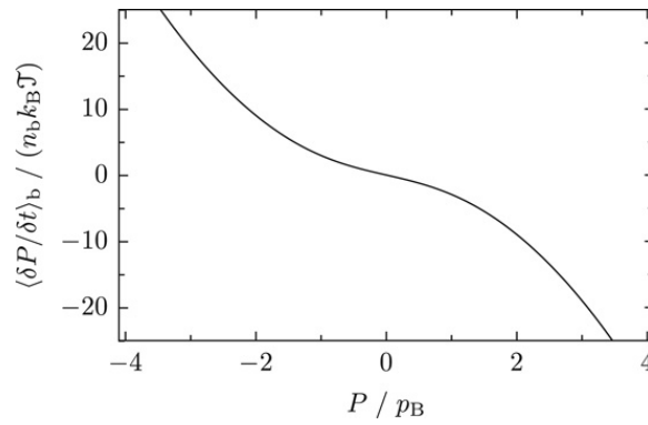
Fig. 1. Nonrelativistic binary collision model. Mean drift force \mathcal{K}(P) = \langle \delta P(t) / \delta t \rangle_b from Eq. (58) with n_b = N/L denoting the number density of the heat bath particles and p_B := M(2k_B \mathcal{T} / m)^{1/2} the characteristic momentum of a Brownian particle (mass M ), surrounded by heat bath particles of mass m and temperature \mathcal{T} .
