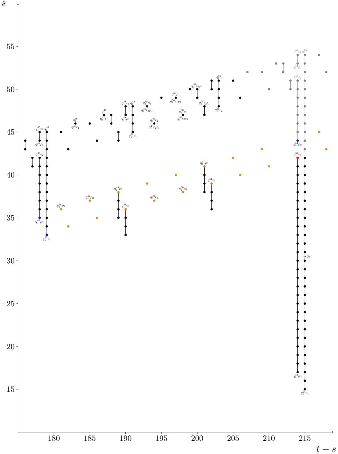
Figure 5-1: The relevant part of H^{s,t}(A) when p = 3 , in the range 175 < t - s < 219 . Vertical black lines indicate multiplication by q_0 . The top and/or bottom of selected q_0 -towers are labelled by the source and/or target, respectively, of the corresponding Bockstein differential.
