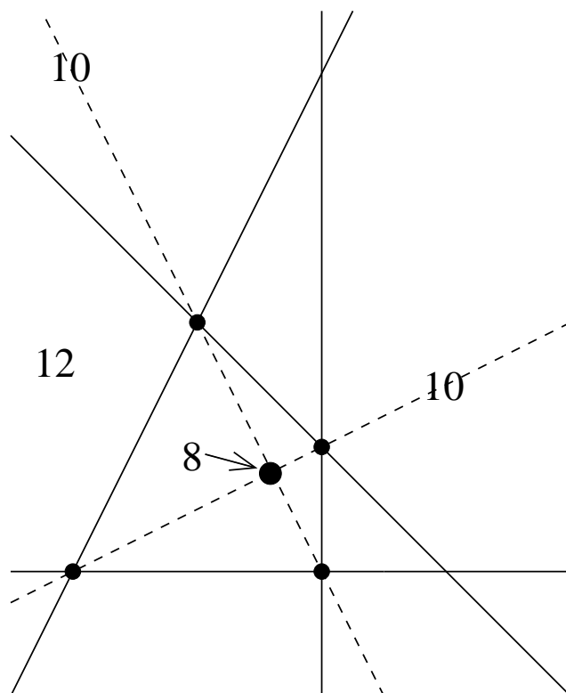
Fig. 2 An example of a polyhedral decomposition \Gamma associated to valid orderings
