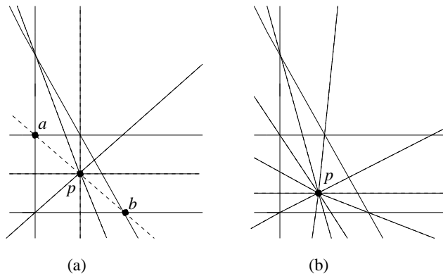
Fig. 1 Two valid order arrangements
